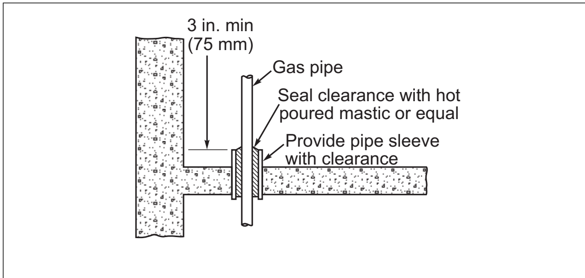
Fig. 2.2.2.4-1. Sealing pipe passing through wet floor.
