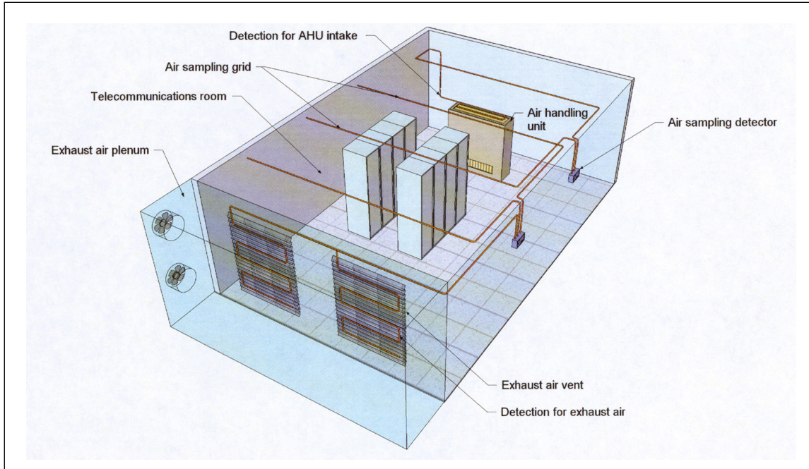
Fig. 3. Very early warning detection system
