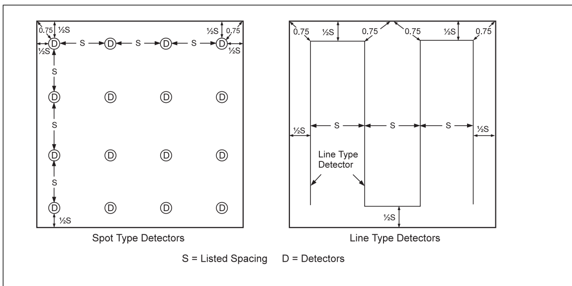
Fig. 2. Spacing of spot-type smoke and heat detectors under a joisted ceiling.
