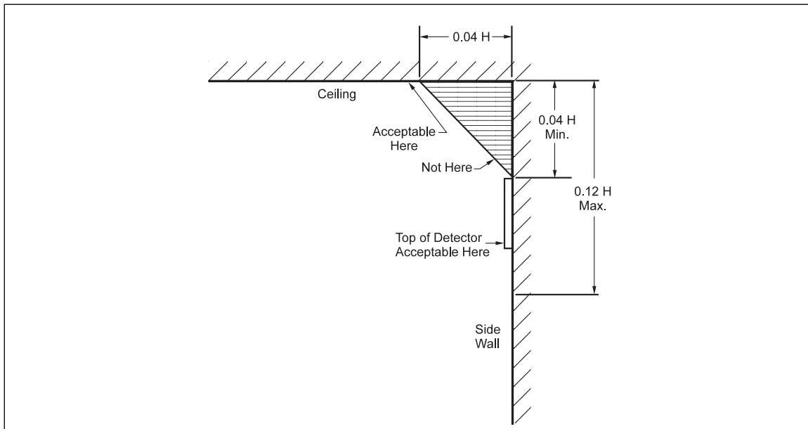
Fig. 1. Recommended location of spot-type heat detectors. Measurements shown are to the closest edge of the detector. H = ceiling height.
