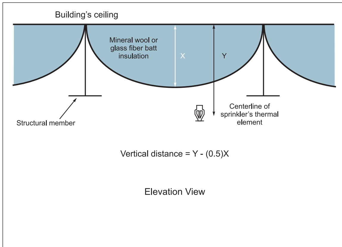
Fig. 25. Vertical distance between ceiling and centerline of sprinkler's thermal element in the presence of mineral wool or glass fiber batt insulation.
