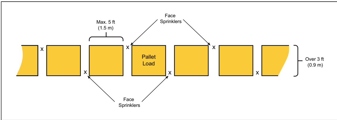
Fig. 2j. Horizontal in-rack sprinkler arrangement for indicated conditions when single-row racks deeper than 3 ft (0.9 m)
