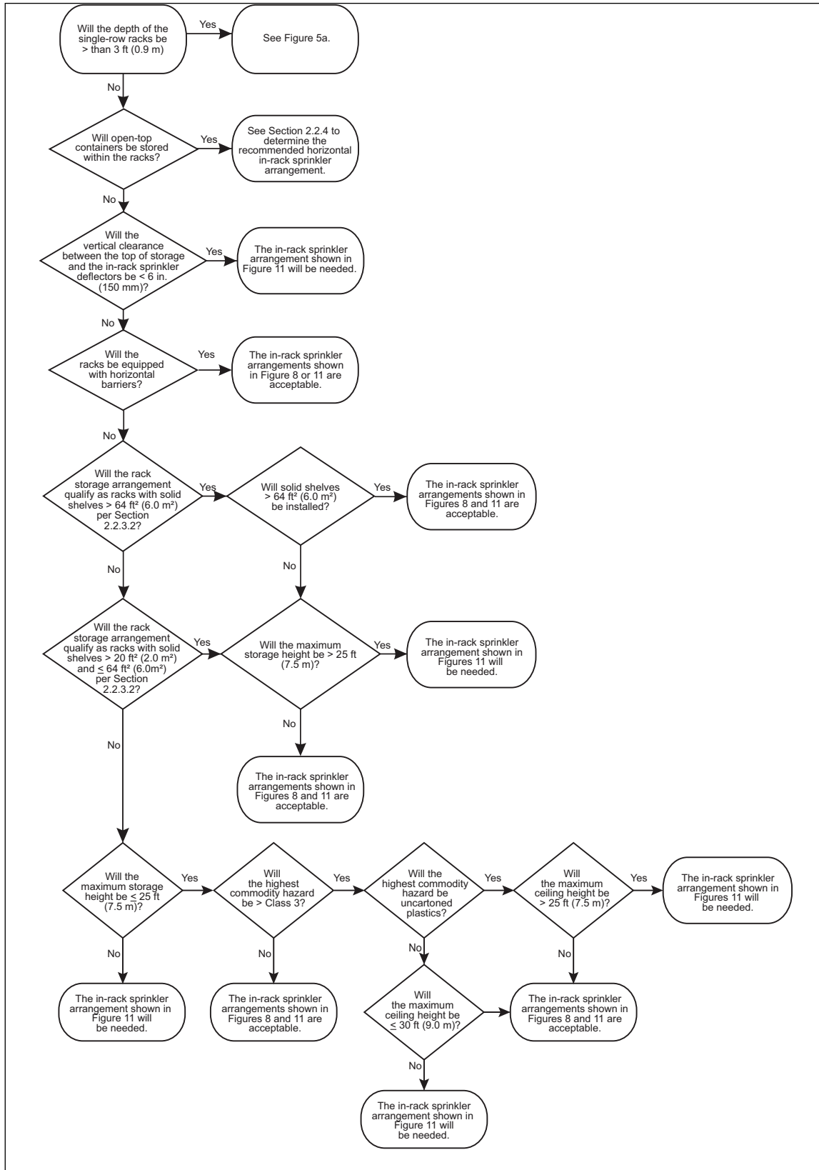
Fig. 5. Recommended horizontal in-rack sprinkler arrangements for single-row racks up to 3 ft (0.9 m) deep
