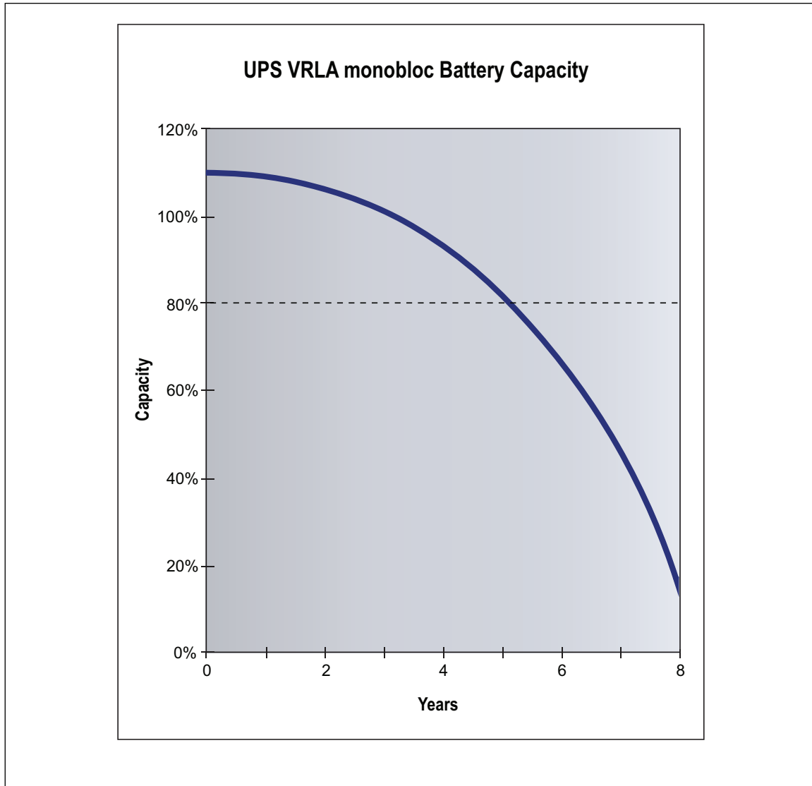
Fig. 4. An example of VRLA battery with design life of 5 years in a controlled temperature environment
