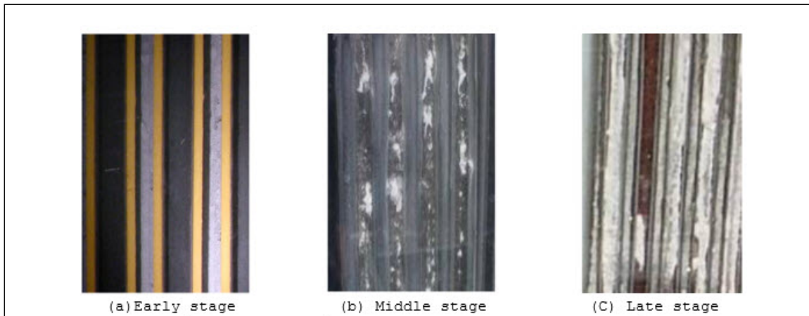
Fig. 1. Sulfation growth at different stages observed through visual inspection
