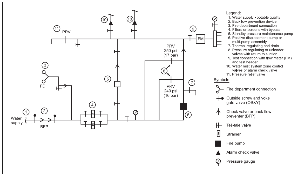
Fig. 2. Typical high-pressure water mist system fire department connection
