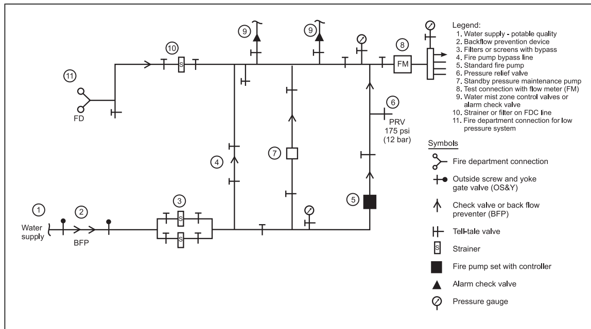
Fig. 1. Typical low-pressure water mist system fire department connection
