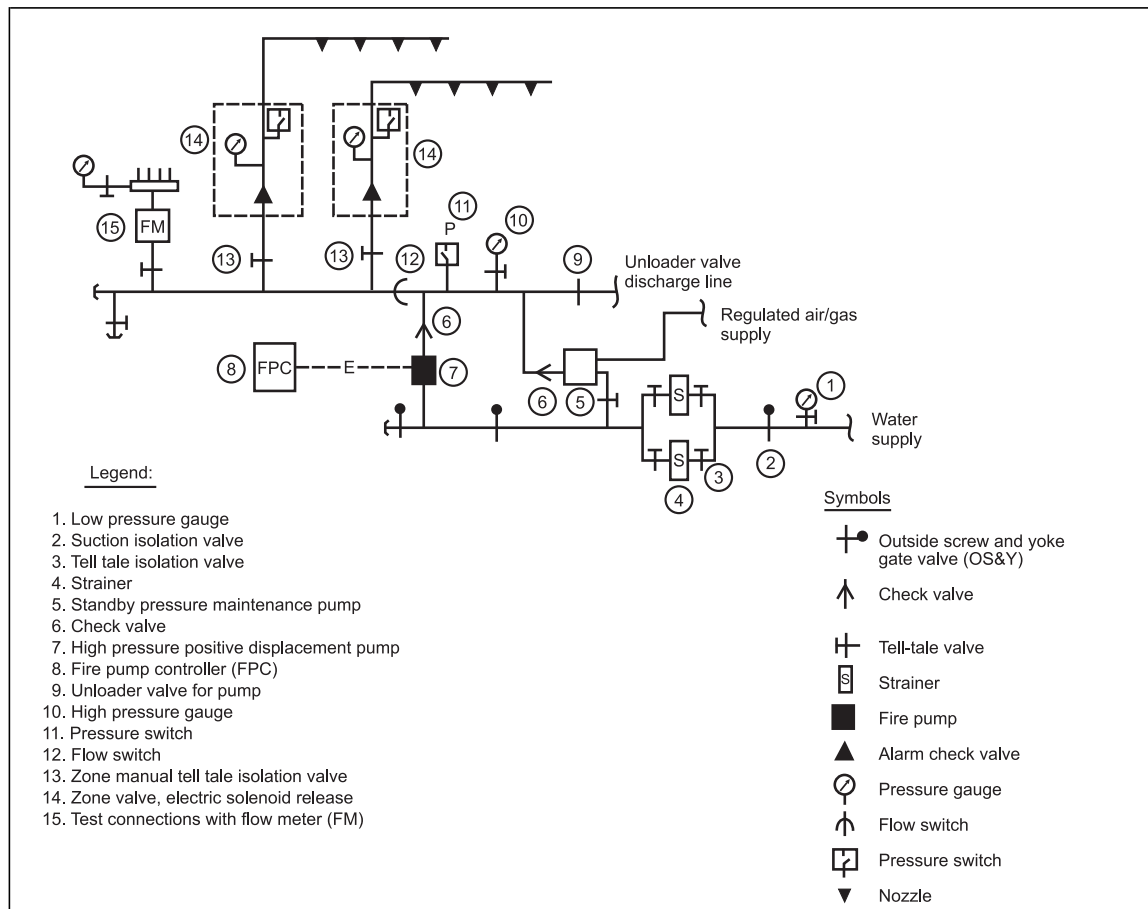
Fig. 4. Schematic of high-pressure water mist system (pump driven)
