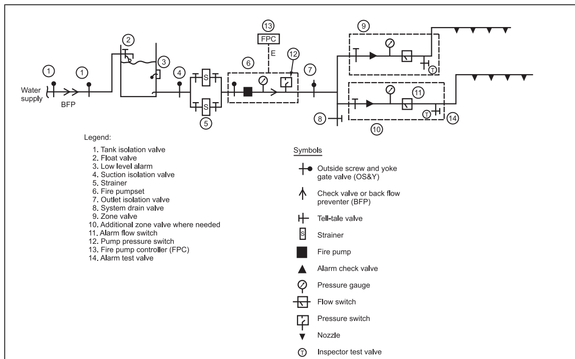
Fig. 3. Schematic of low-pressure water mist system (pump driven)
